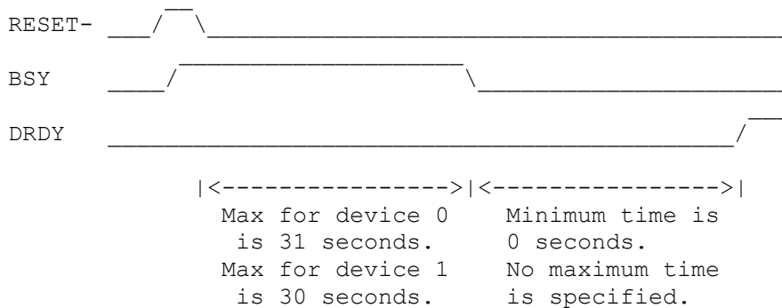
Figure 8 - BSY and DRDY timing for power on and hardware resets
