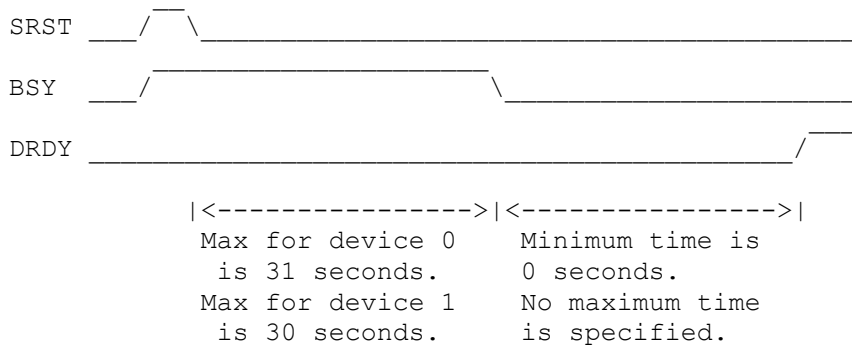
Figure 9 - BSY and DRDY timing for software reset
