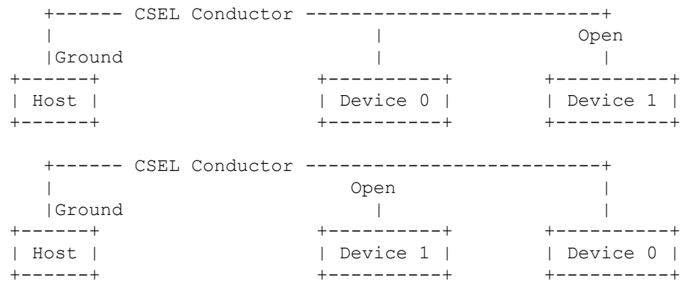
Figure 4 - Cable Select Example
