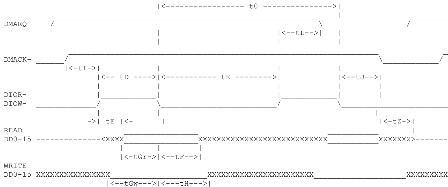
Figure 12 - Multiword DMA Data Transfer (Part 1 of 2)
